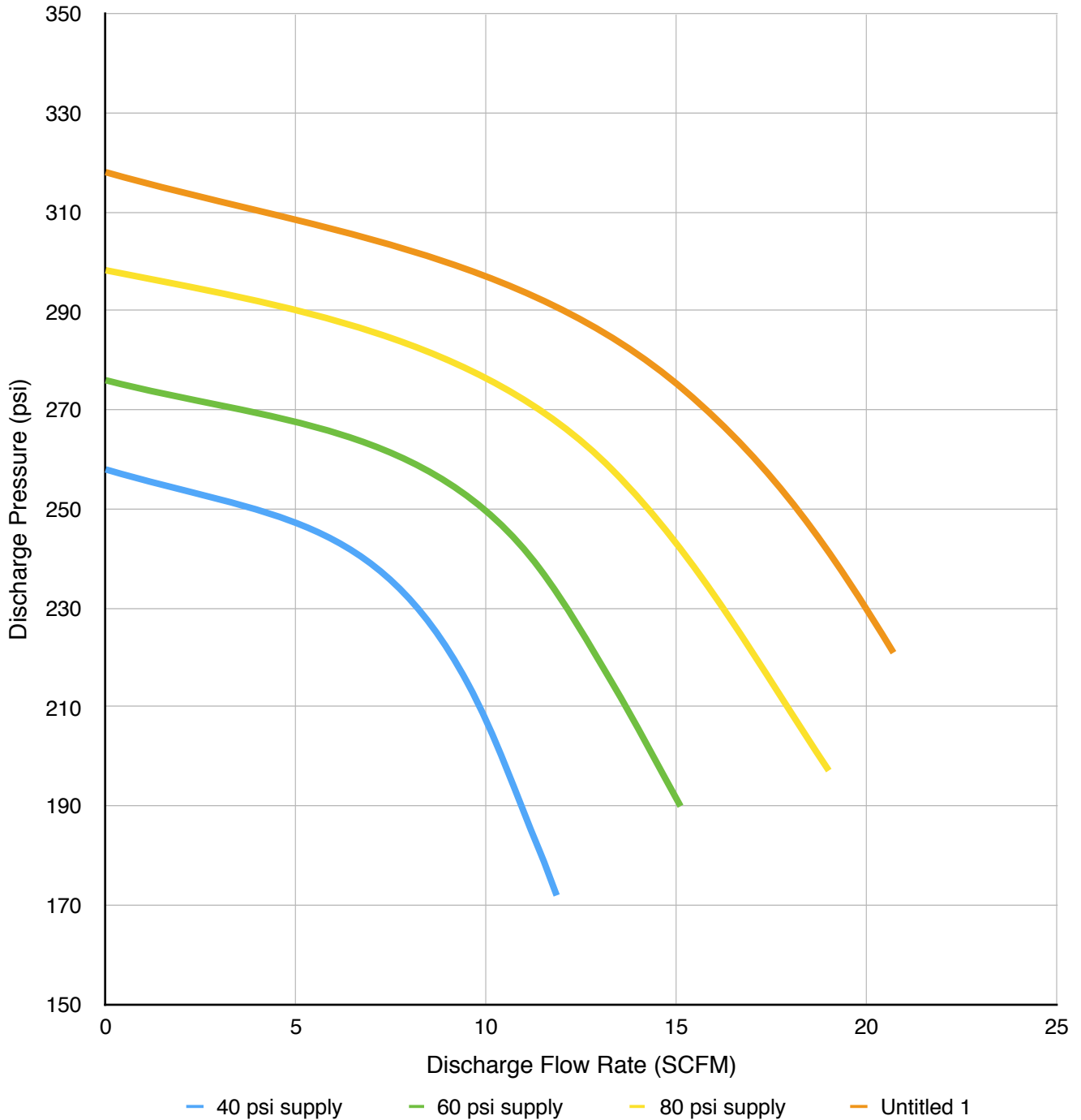
53AAV34 - Discharge Pressure VS Flow Rate Drive Pressure 80 psi & Gas Supply Pressure Varies
