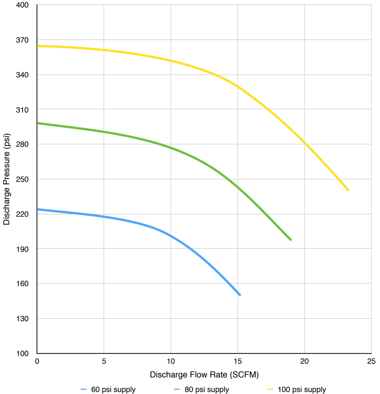
53AAV34 - Discharge Pressure VS Flow Rate Drive Pressure & Gas Supply Pressure Equal
