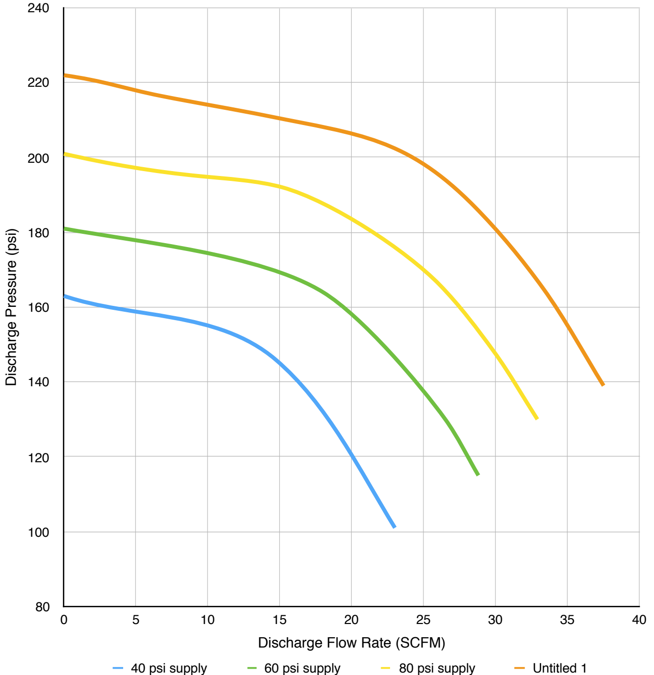
54AAV24 - Discharge Pressure VS Flow Rate Drive Pressure 80 psi & Gas Supply Pressure Varies
