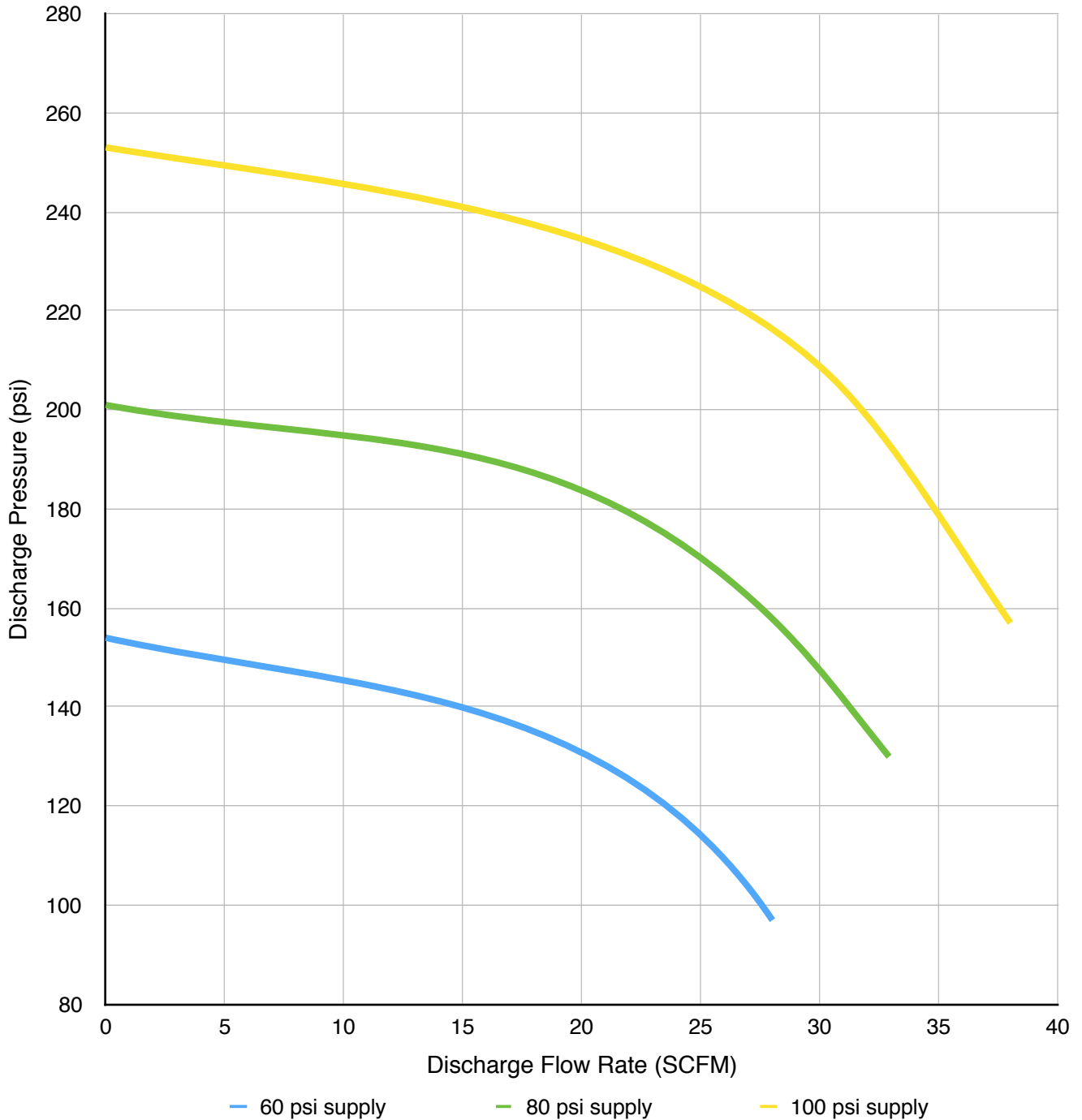
54AAV24 - Discharge Pressure VS Flow Rate Drive Pressure & Gas Supply Pressure Equal
